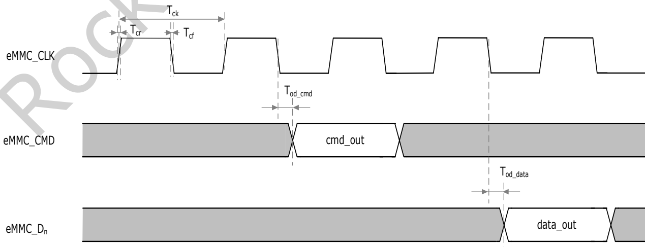
Fig.4-2 eMMC output mode timing
