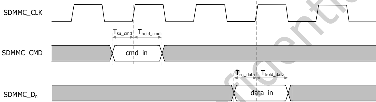
Fig.4-5 SDMMC input mode timing
