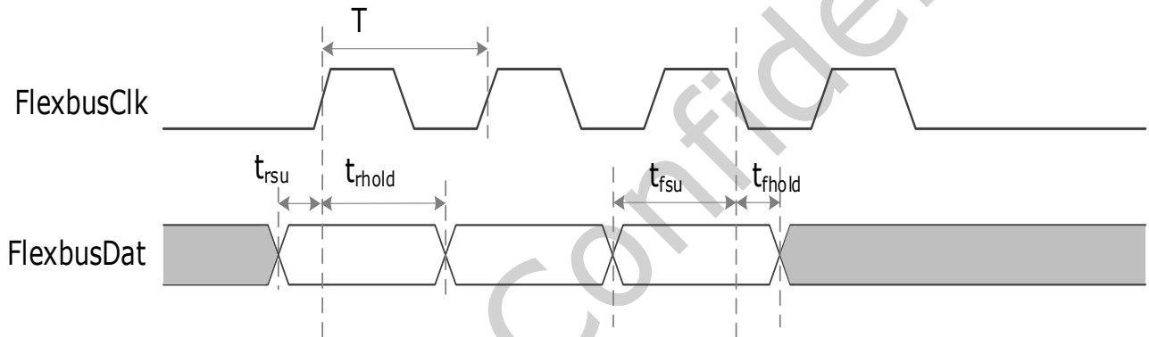
Fig.4-15 Flexbus interface slave mode timing
