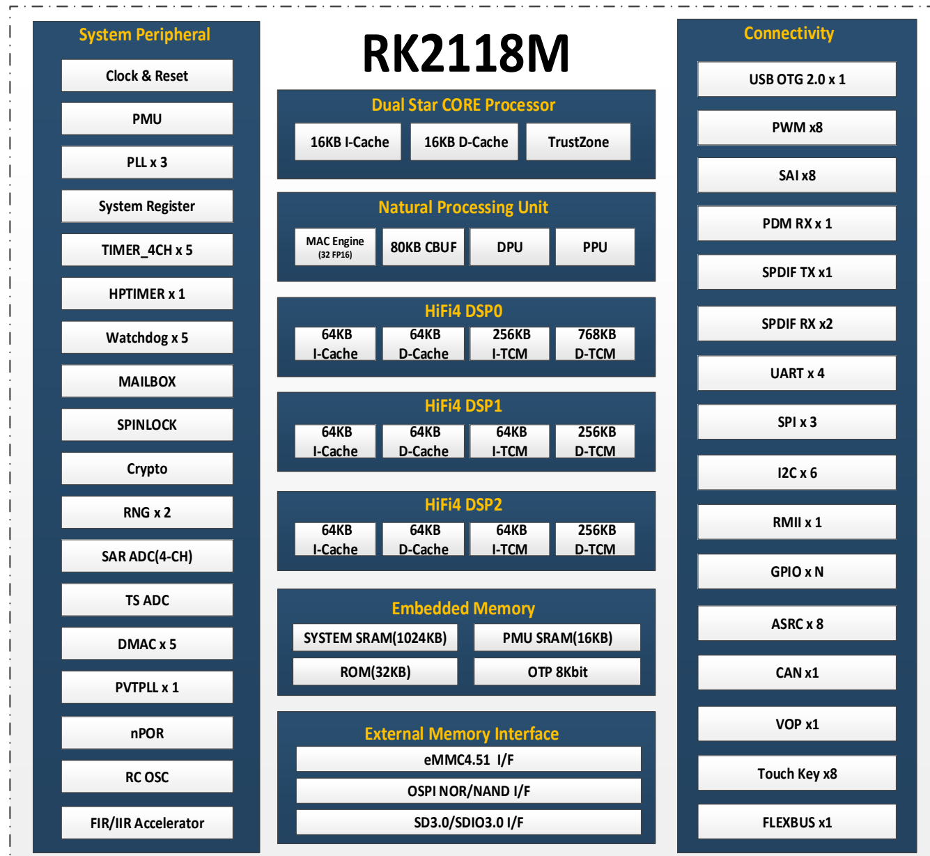
Fig.1-1 RK2118M Block Diagram
