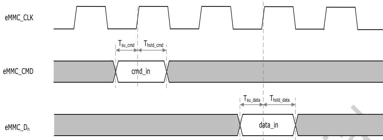
Fig.4-3 eMMC input mode timing
