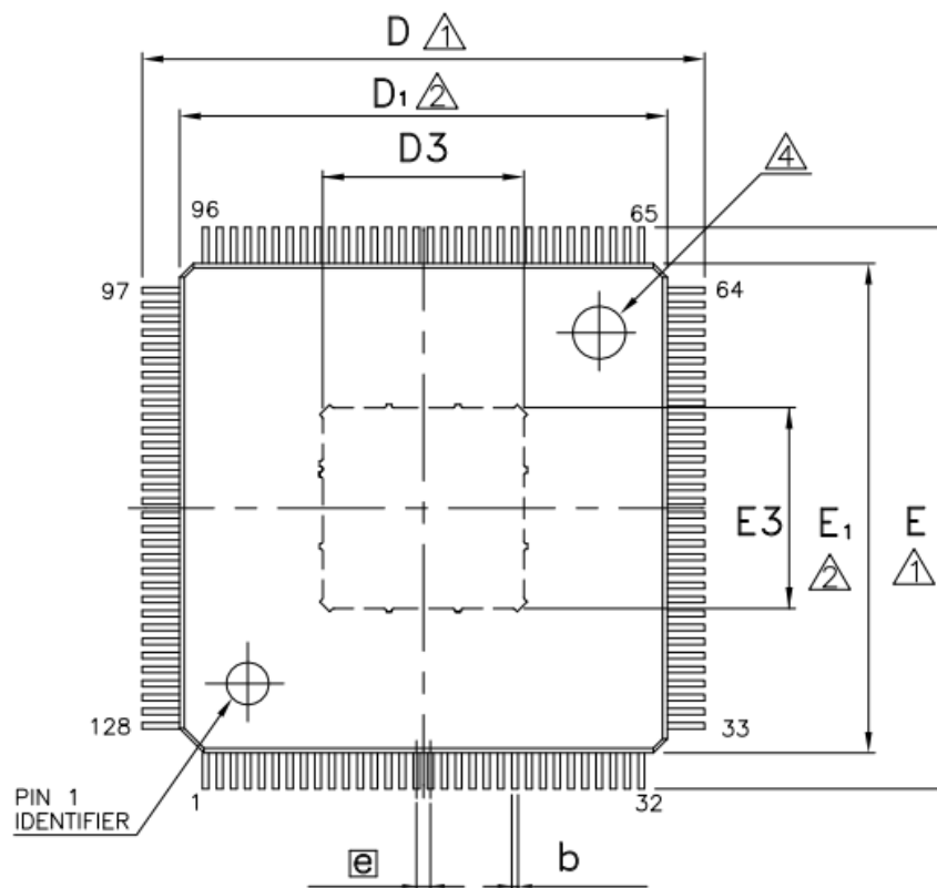
Fig.2-2 RK2118M Package Top View
