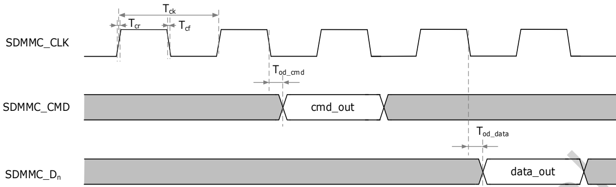
Fig.4-4 SDMMC output mode timing
