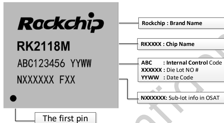
Fig.2-1 RK2118M Package Definition
